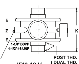
IF*2-12 V
